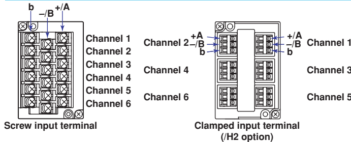
Channel location on the input terminals
