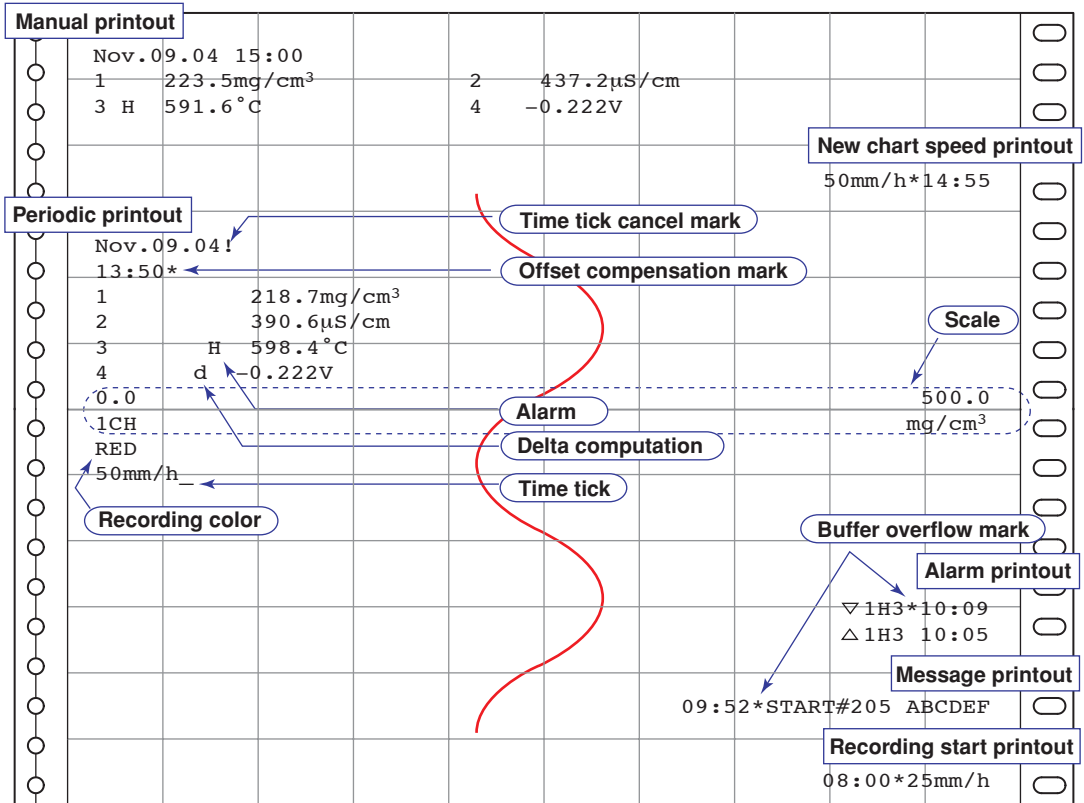
Printout Description Figure (Pen Model)
